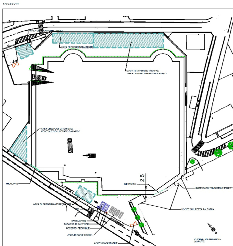
LAYOUT 2
